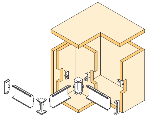
Horizontal drawer "C" profile.
