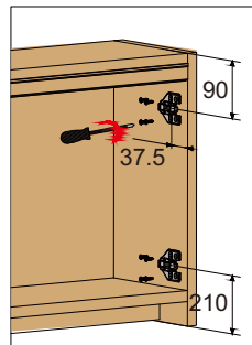
Install the hinge plates.
